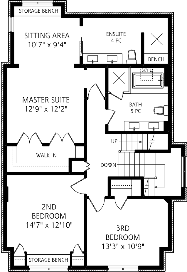
SECOND FLOOR 1,185 SQUARE FEET
