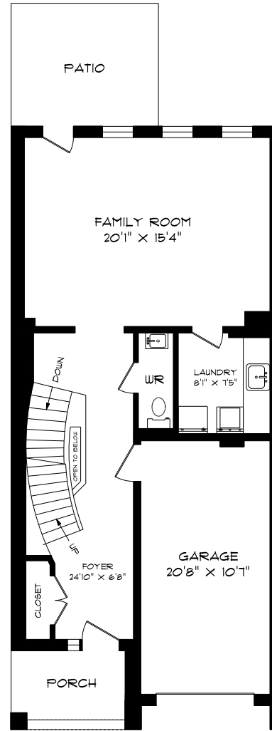
GROUND FLOOR 138 SQUARE FEET
