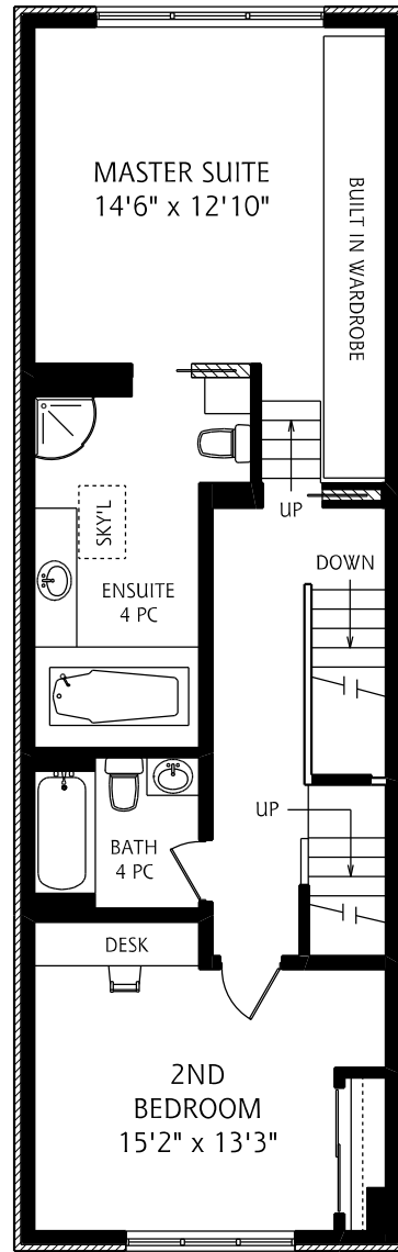
SECOND FLOOR 910 SQUARE FEET
