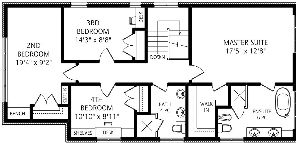
SECOND FLOOR 1,190 SQUARE FEET
