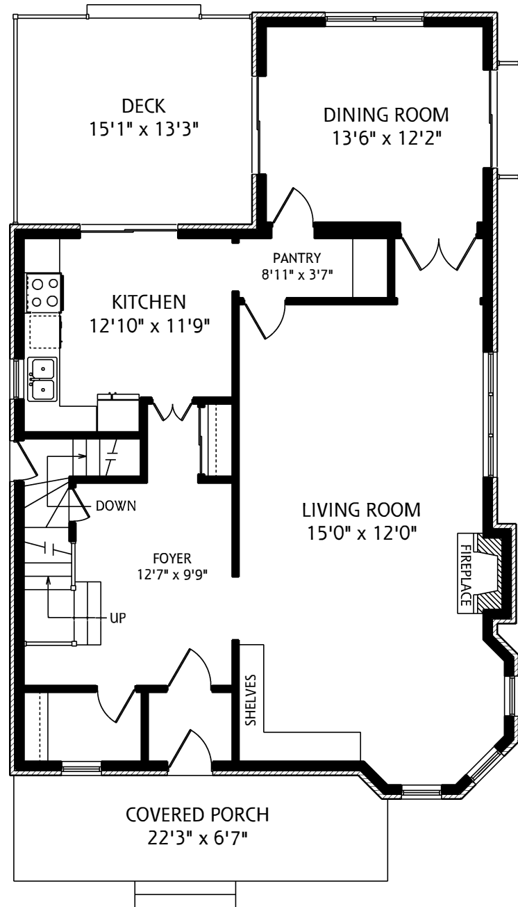
MAIN FLOOR 1,275 SQUARE FEET
