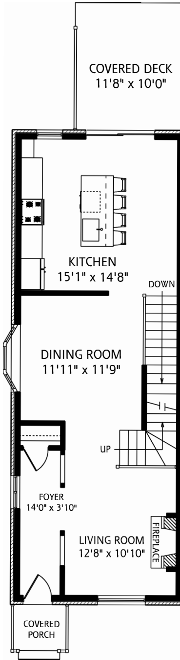
MAIN FLOOR 765 SQUARE FEET
