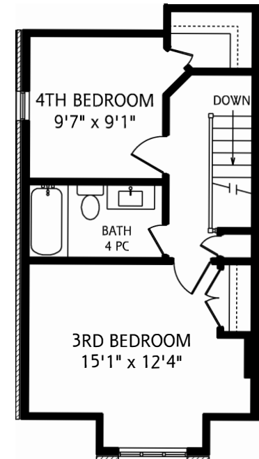
THIRD FLOOR 475 SQUARE FEET
