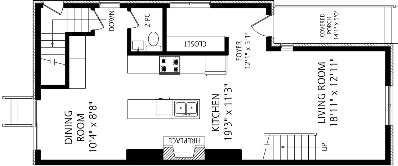
MAIN FLOOR 780 SQUARE FEET
