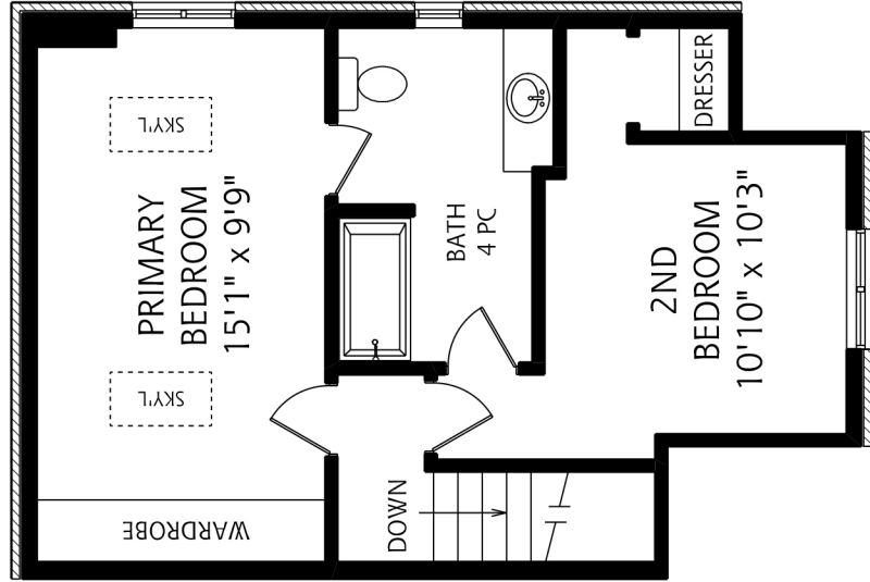
SECOND FLOOR 530 SQUARE FEET
